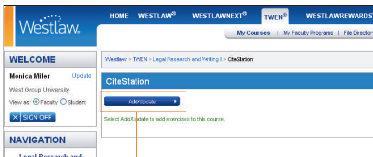
Figure 1. CiteStation page
